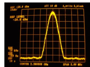
SOQPSK-TG Configuration
